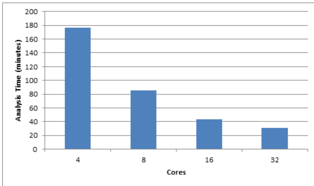
Data set 3: Emails - 768K documents, 11.7 GB total text
